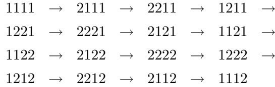
Figure 5.3 Colour classes visited in a shortest path between a (1, 1, 1, 1) -colouring and a (1, 1, 1, 2) -colouring of G_4 .
