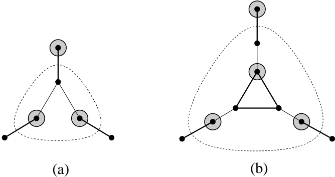
Figure A.1 (a) an AND sliding-token gadget, and (b) an OR sliding-token gadget.
