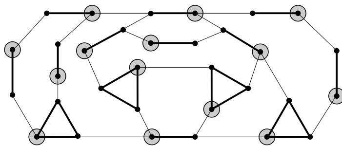
Figure 5.2 An example of a restricted instance graph together with a standard token configuration.
