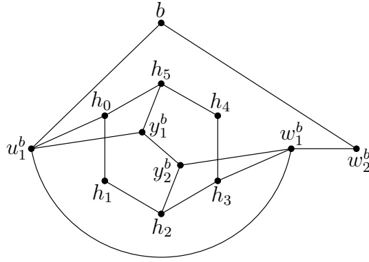
Figure 3.2 The subgraph of G' added around a vertex b \in G_B \setminus S_B , together with the 6-cycle S .
