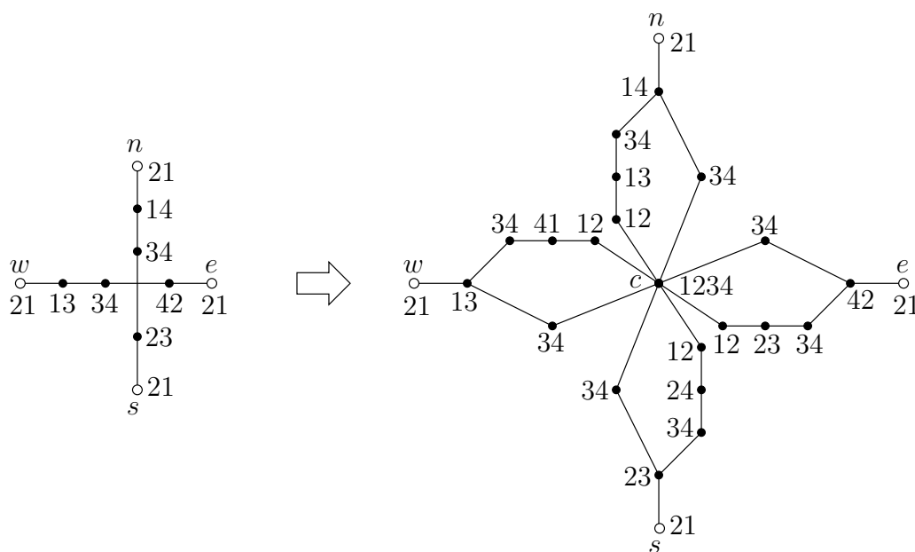
Figure 5.4 A crossing component corresponding to two (1,2) -forbidding paths.
