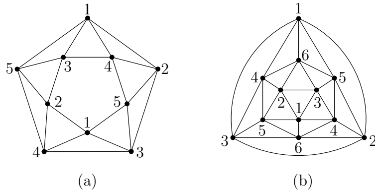
Figure 2.2 (a) a planar graph with a frozen 5-colouring, and (b) a planar graph with a frozen 6-colouring.
