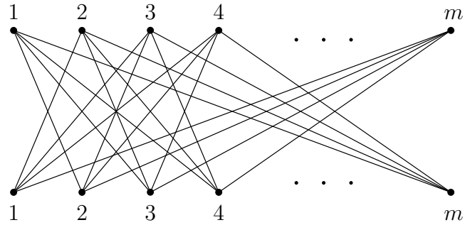
Figure 2.1 The graph L_m together with a frozen m -colouring.
