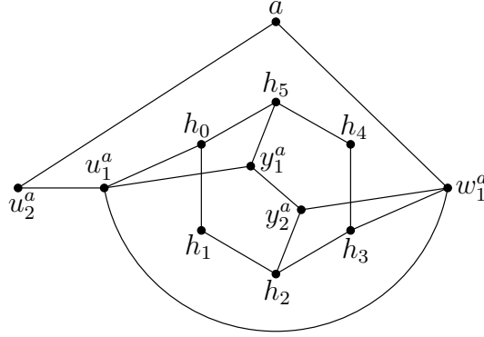
Figure 3.1 The subgraph of G' added around a vertex a \in G_A \setminus S_A , together with the 6-cycle S .
