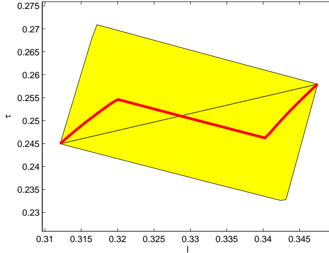
Figure 3.2: Optimal policy with log-quadratic utility
