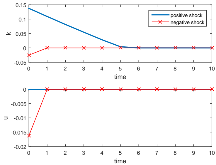
Figure 2.2: Impulse Response Functions (3 standard dev. shock)
