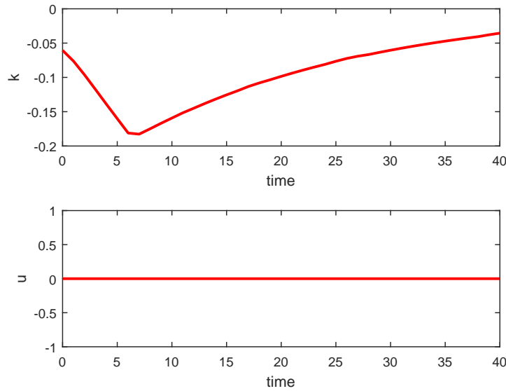
Figure 2.6: Impulse Response Functions (3 standard dev. persistent shock)
